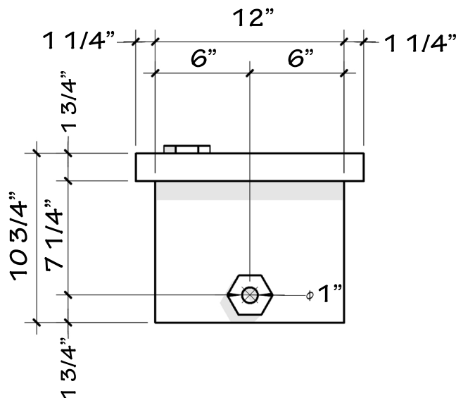
INLET
